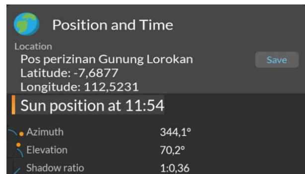
Figure 5. Sun Position Gunung Lorokan
