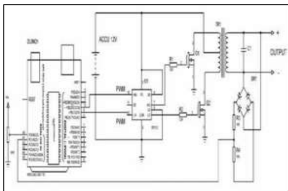
Gambar 4. Rangkaian Driver Mosfet
