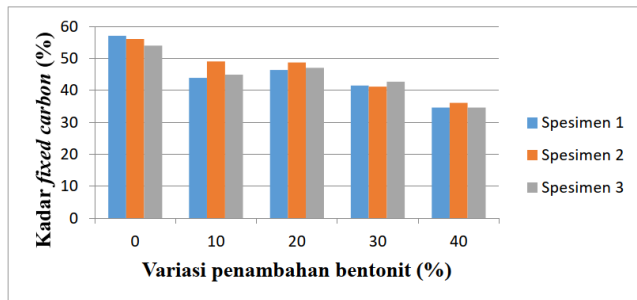
Fig. 5. Graph of fixed carbon
